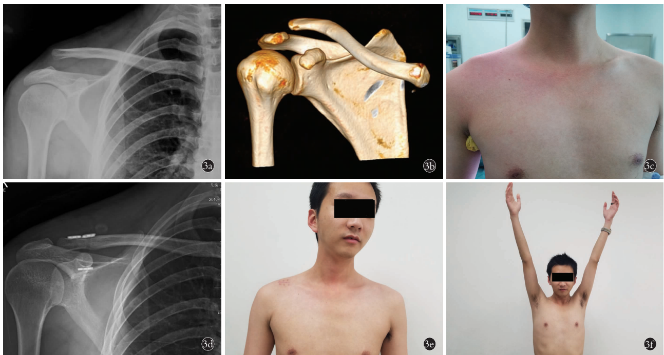
图 3 患者,男,26岁,平地跌伤右肩锁关节脱位 3a. 术前 X 线片示右肩锁关节脱位 Rockwood III 型 3b. 伤后 CT 排除喙突骨折 3c. 术前肩部琴键征阳性 3d. 术后 2 d 的 X 线片示关节复位 3e. 术后 5 周,肩部外形恢复,见较小切口瘢痕 3f. 术后 5 周功能完全恢复 Fig.3 A 26-year-old male patient with right acromioclavicular joint dislocation due to flat injury 3a. X-ray before operation showed dislocation of right acromioclavicular joint of Rockwood type III 3b. Exclusion of coracoid fracture by CT after injury 3c. Positive sign of piano keys in shoulder before operation 3d. X-ray at 2 days after operation showed reduction of joint 3e. At 5 weeks after operation, the appearance of shoulder recovered, and the scar of smaller incision was seen 3f. Complete recovery of function at 5 weeks after operation
